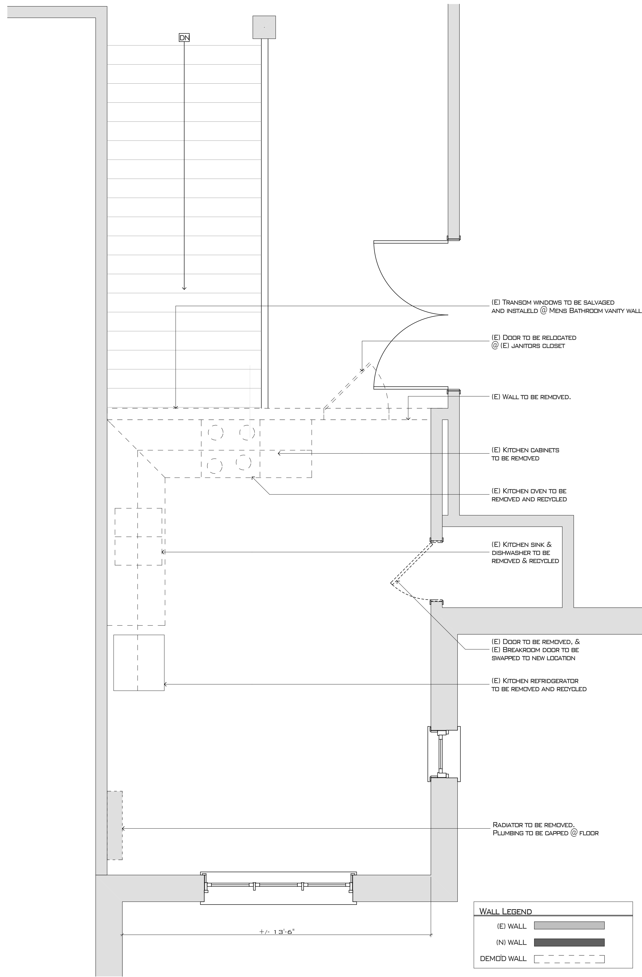
DEMO FLOOR PLAN SCALE: 1/2" = 1'-0"
