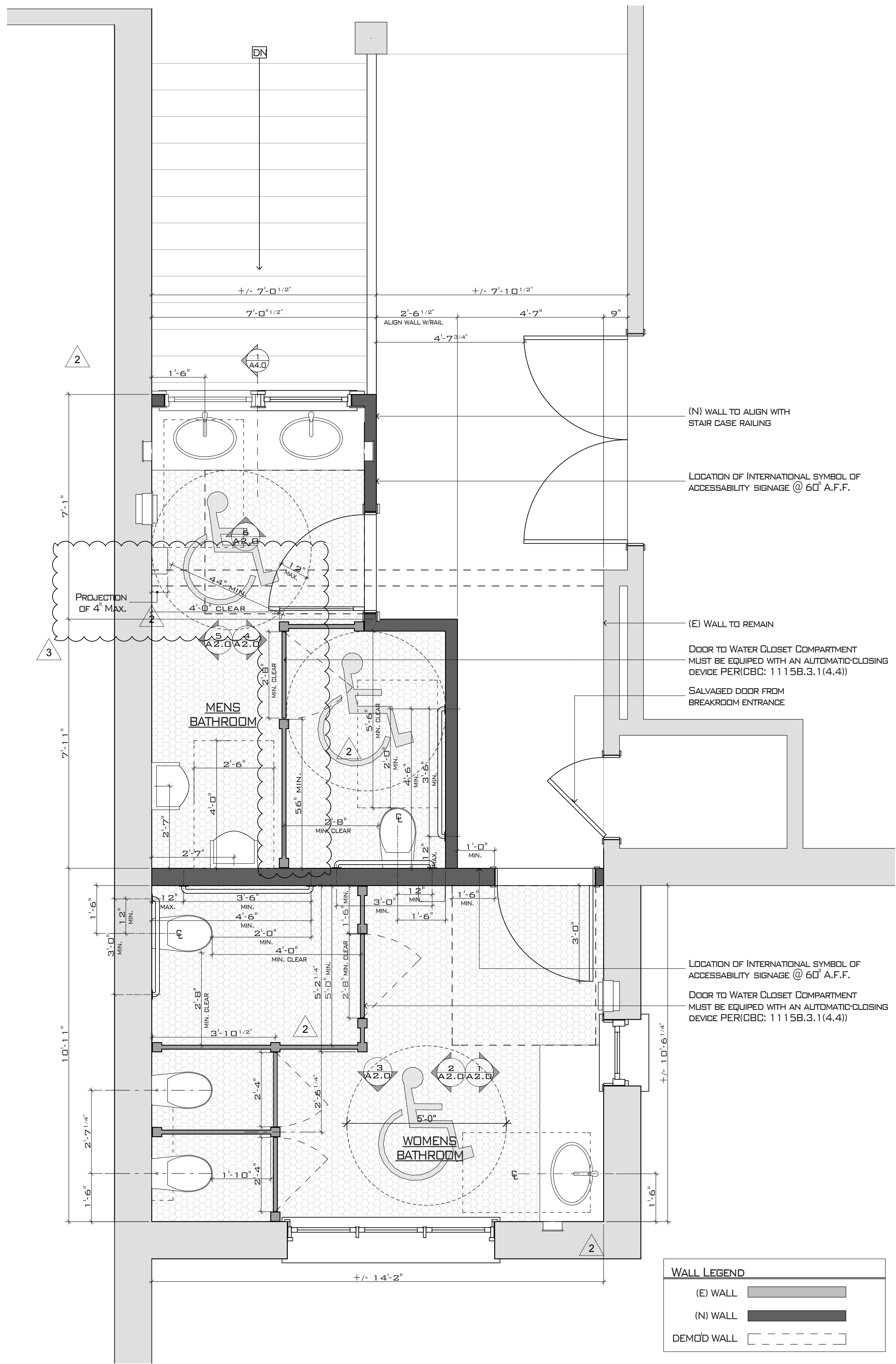
RESTROOM FLOOR LAYOUT SCALE: 1/2" = 1'-0"
