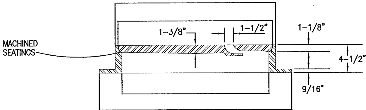
SECTION THRU FRAME AND COVER
