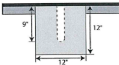
Center Anchor
